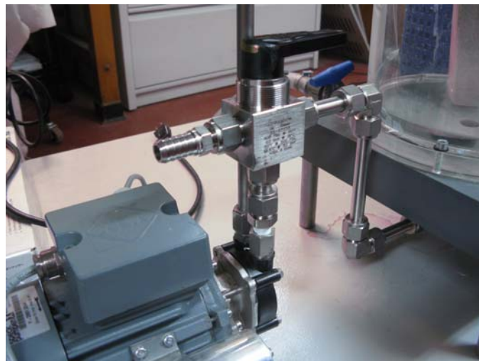
Figure 1. Three way valve modification for flushing and priming the recirculating pump.
